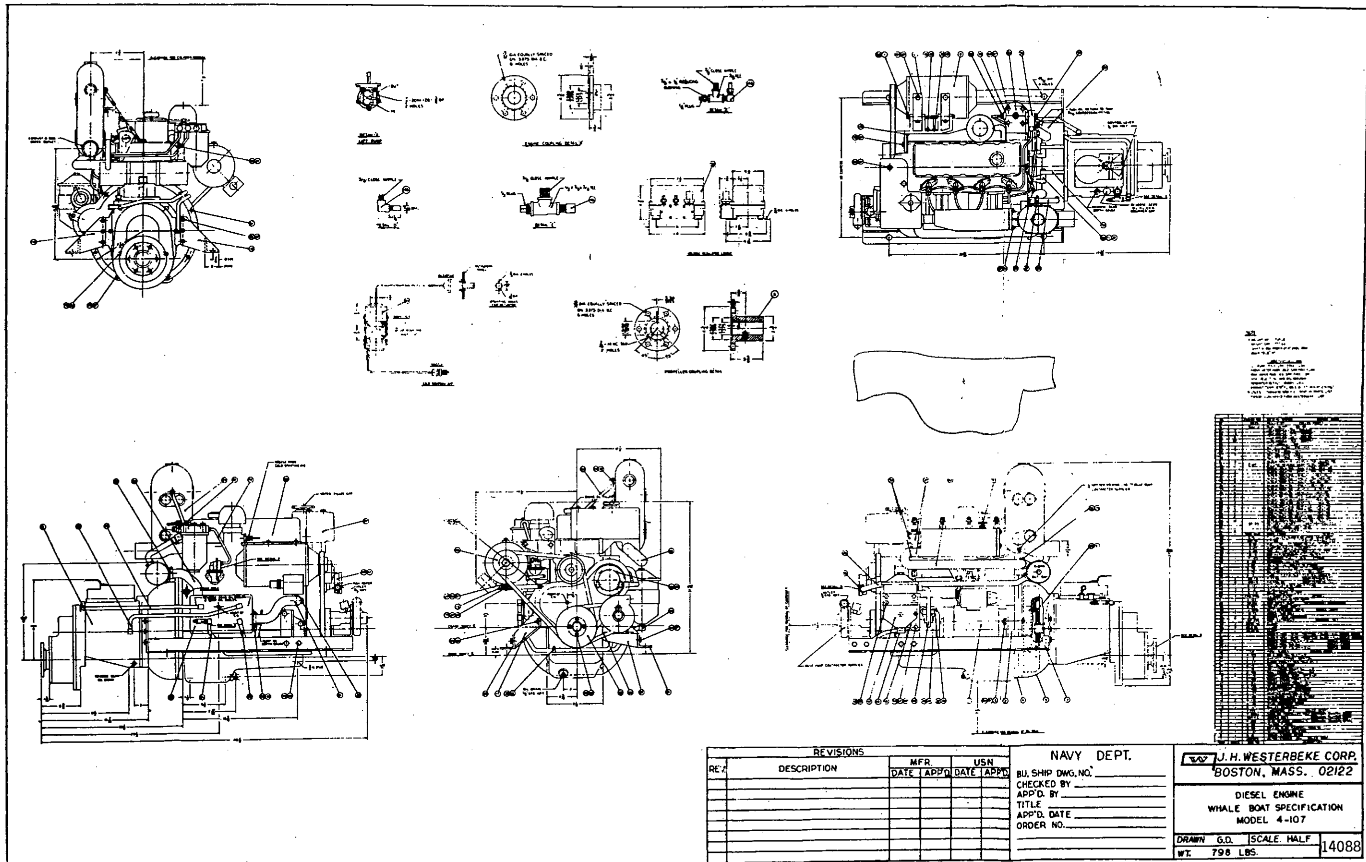
Fig. 7—Installation Drawing of Westerbeke Four-107
